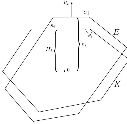
Figure 4.1: Notation used for K and a parallel set E .
