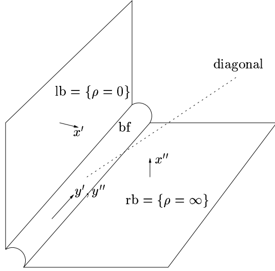
FIGURE 1. The blown up space \overline{M}_b^2
